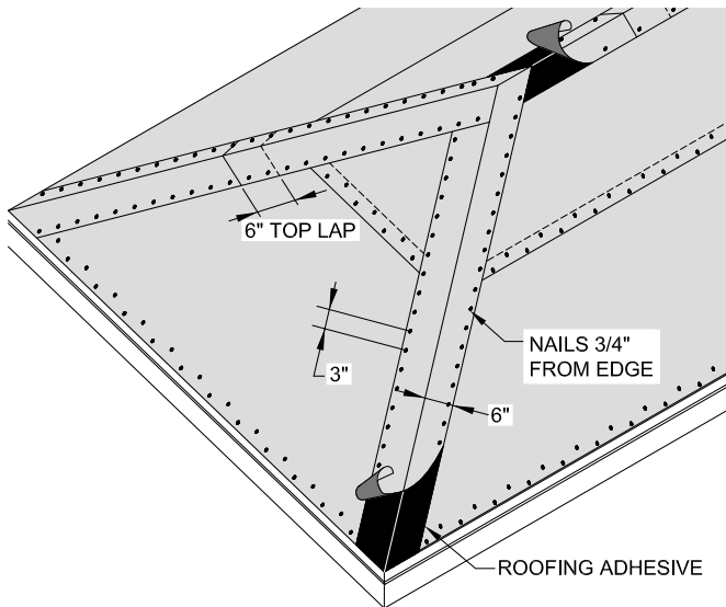
Figure 4 - Hips and Ridges: Exposed Fastener Installation
