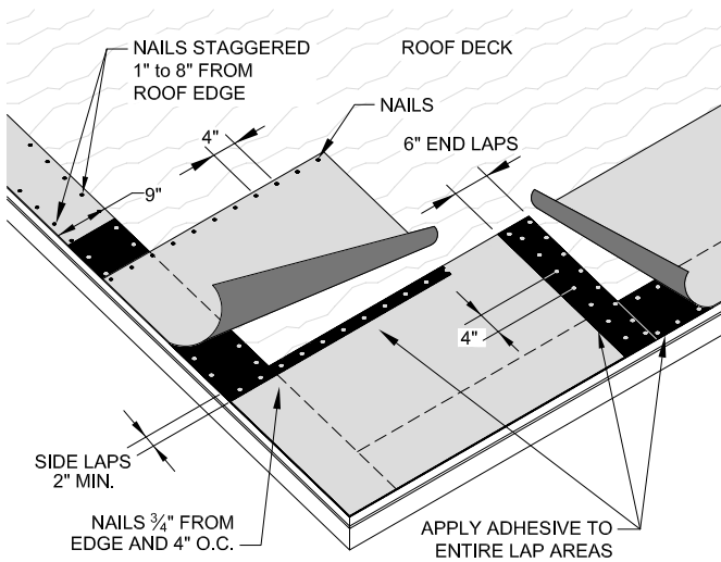
Figure 1 - Application of CHROMA Cap: Concealed Fastener Installation
