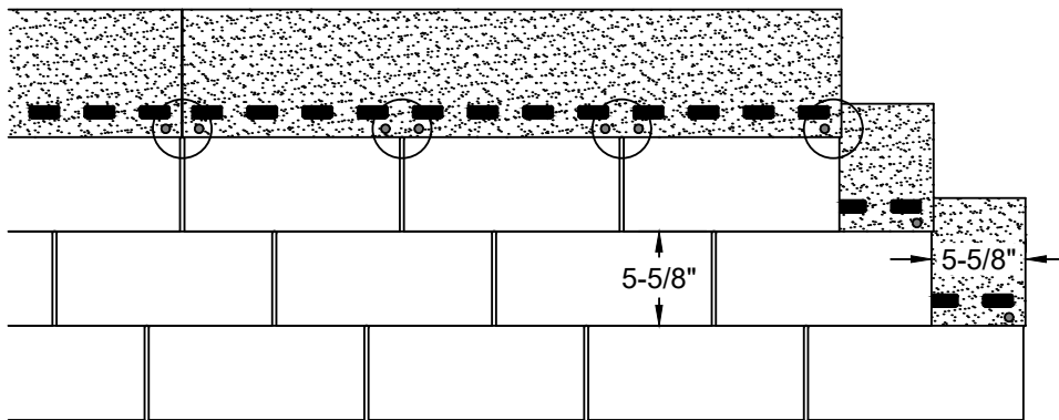
3-TAB 6 NAIL PATTERN
