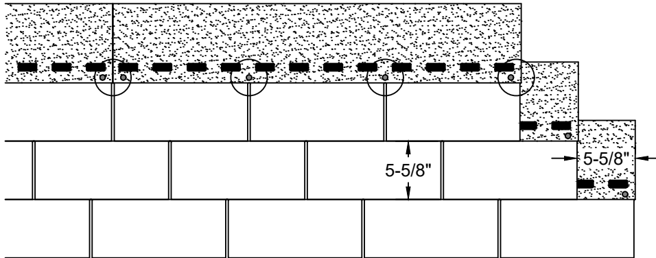
3-TAB 4 NAIL PATTERN
