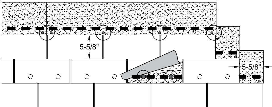
HAND-SEALING 3-TAB SHINGLES
